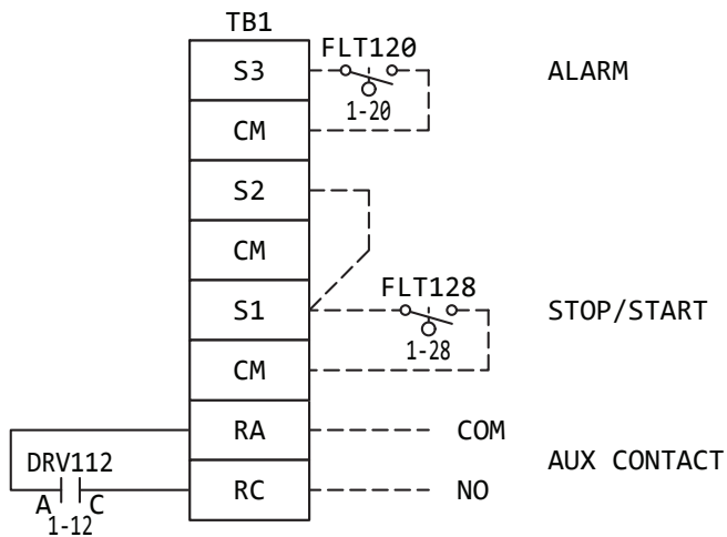
2 FLOAT CONNECTION
