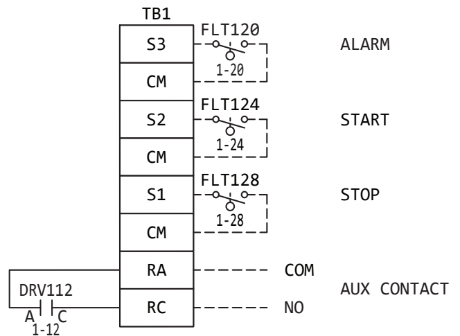
3 FLOAT CONNECTION
