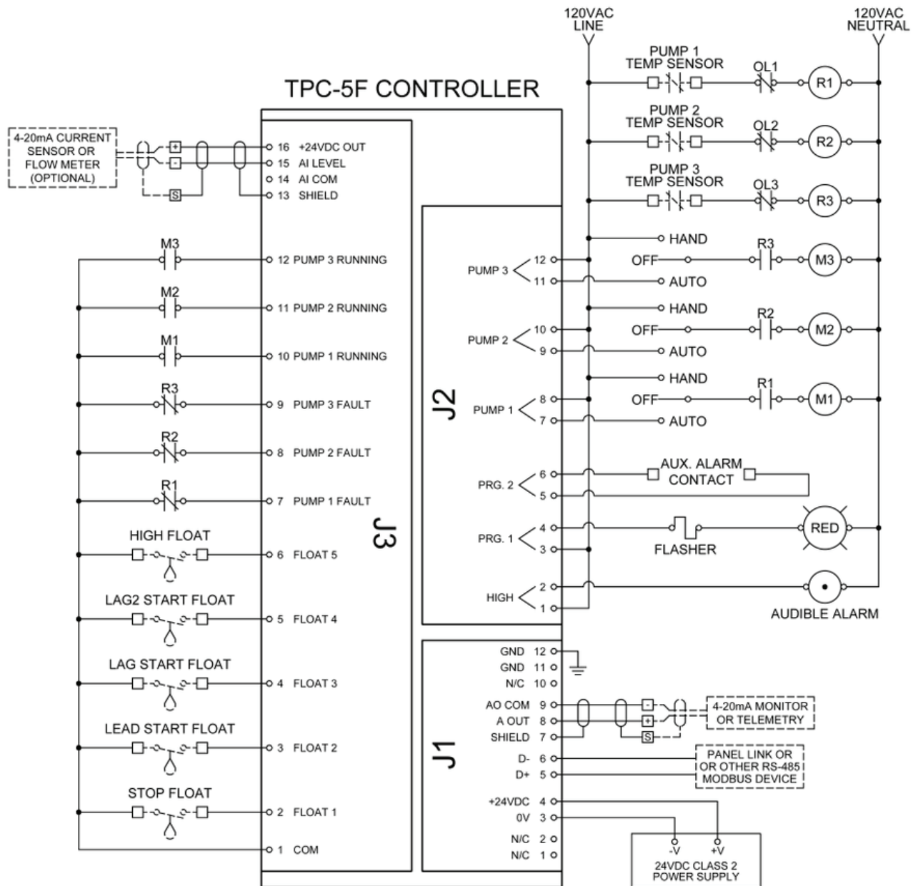
EXAMPLE DEPICTS FLOAT CONFIGURATION 5
