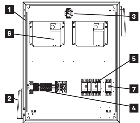
VARIOspeed® 3R Duplex (240V model)
