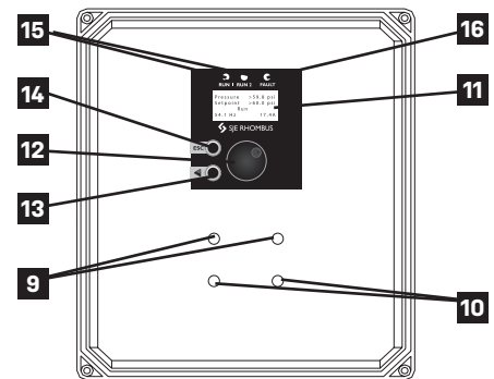
VARIOspeed® 3R Duplex door & display (mounted internally)
