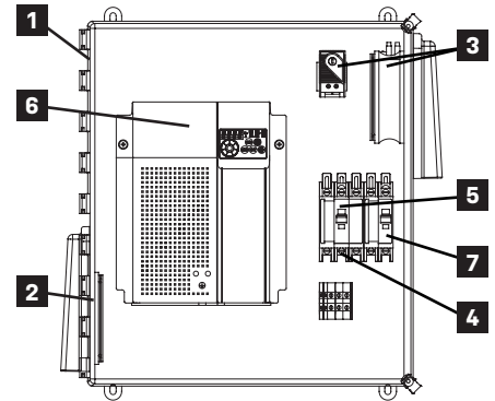
VARIOspeed® 3R (240V model)
