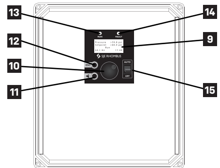
VARIOspeed® 3R door & display (mounted internally)
