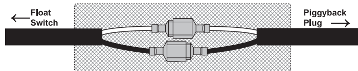
Center Heat Shrink on Terminal Connection
